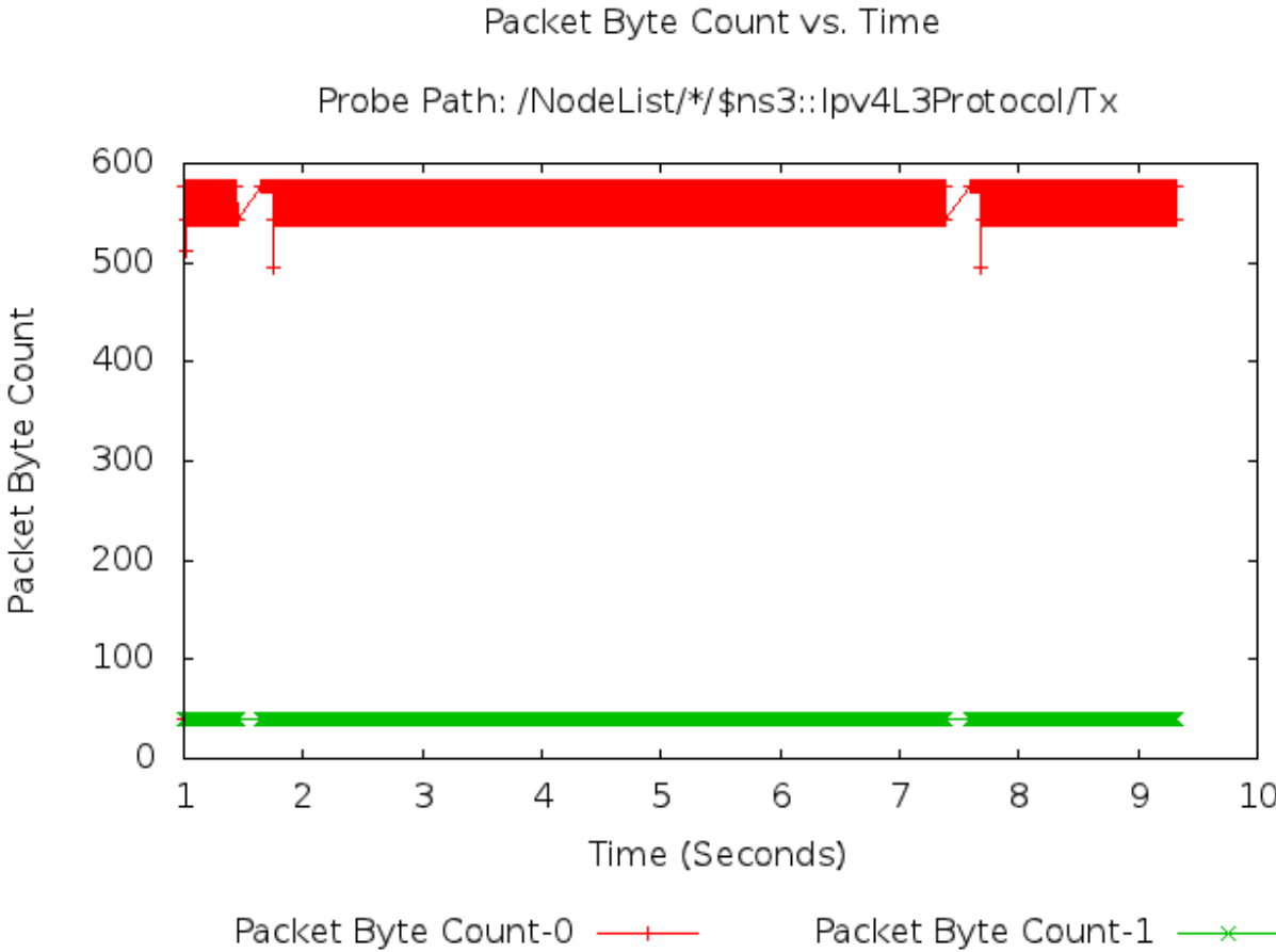
Fig. 3: 2-D Gnuplot Created by seventh.cc Example.
