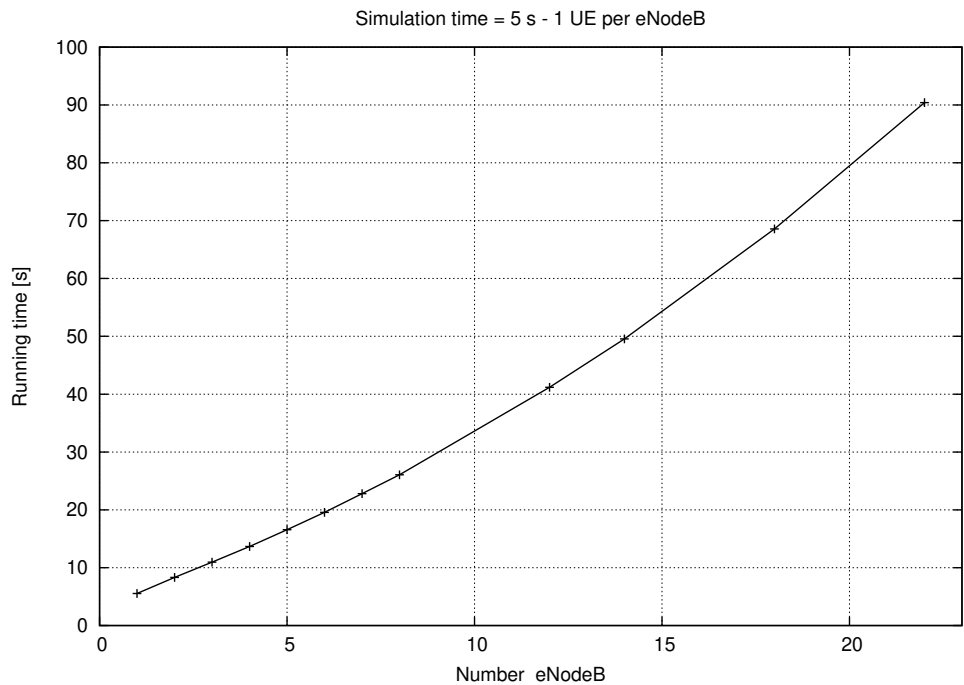
Fig. 107: Running time
